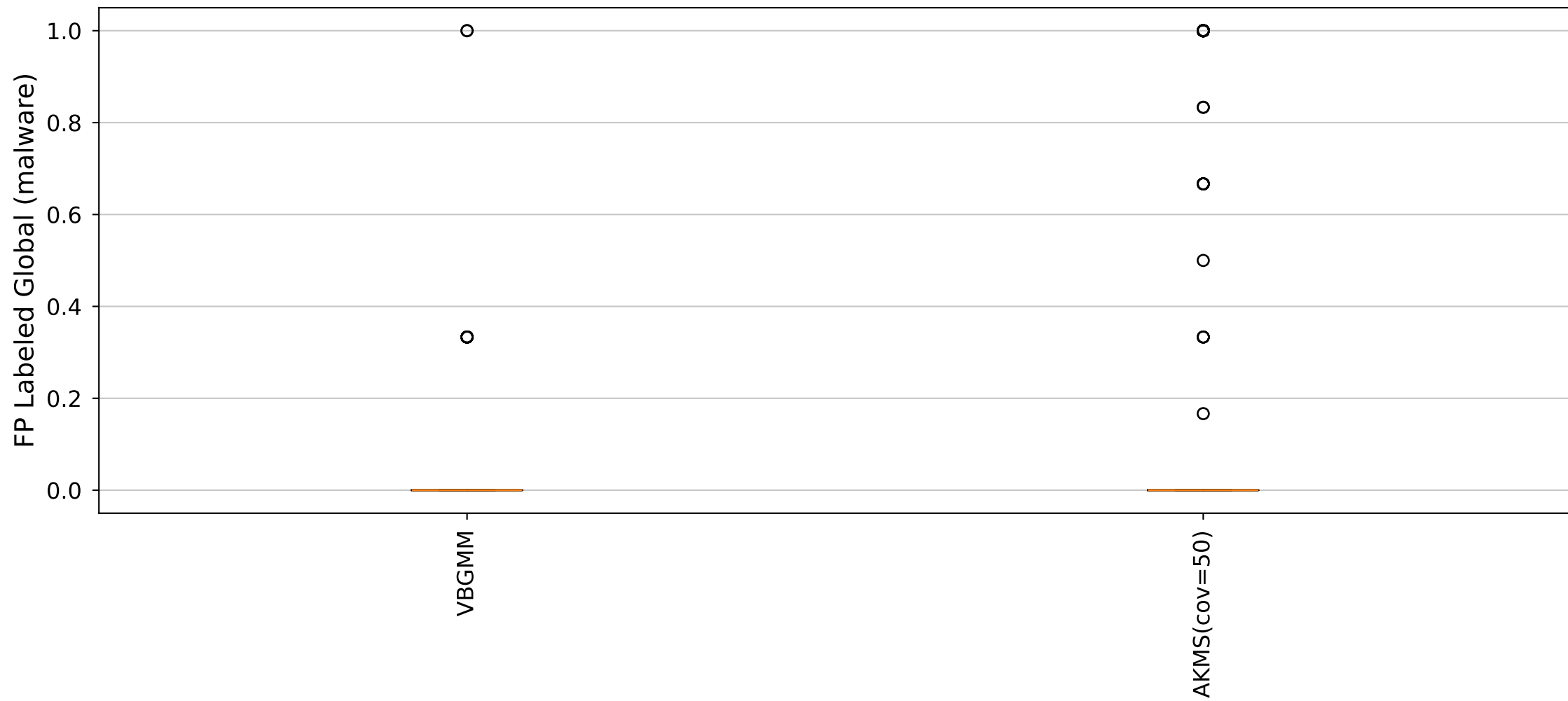
YARA Rules FP Labeled Global (malware) Distribution (Cluster3_Size53 dataset)
